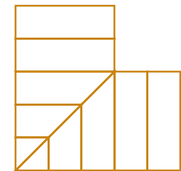
4 x 12 Fullnose Corner Detail
